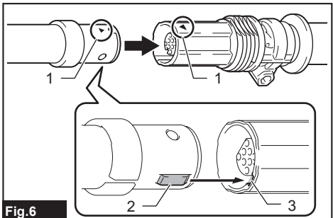
Fig.6 ▶ 1. Triangle mark 2. Tongue 3. Groove
